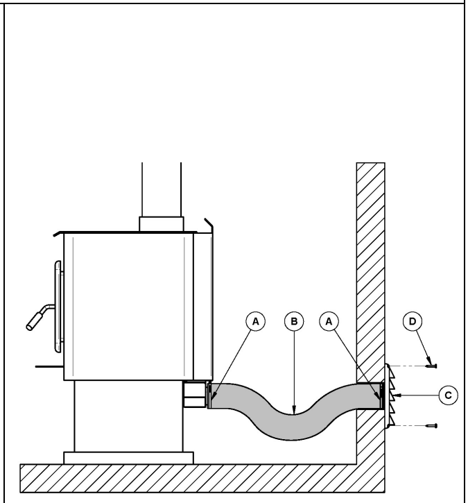
A- Clamp, B- 5" insulated pipe (not included), C- Air intake cap, D- Intake cap attachment screws (not included).
