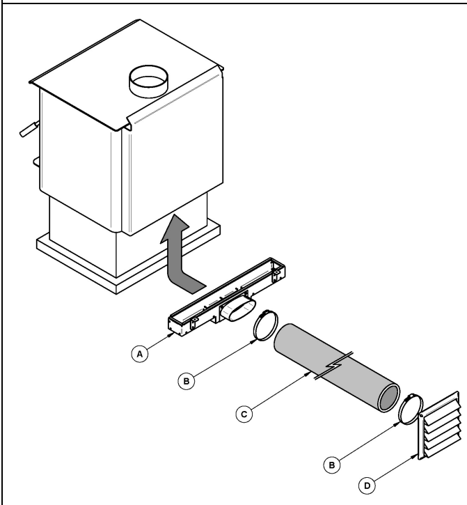
A- Air intake housing, B- Clamp, C- 5" insulated pipe (not included), D- Air intake cap.
