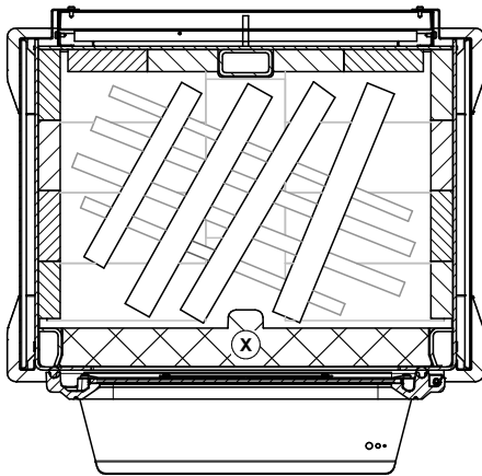
Figure 15: Start-up fuel
