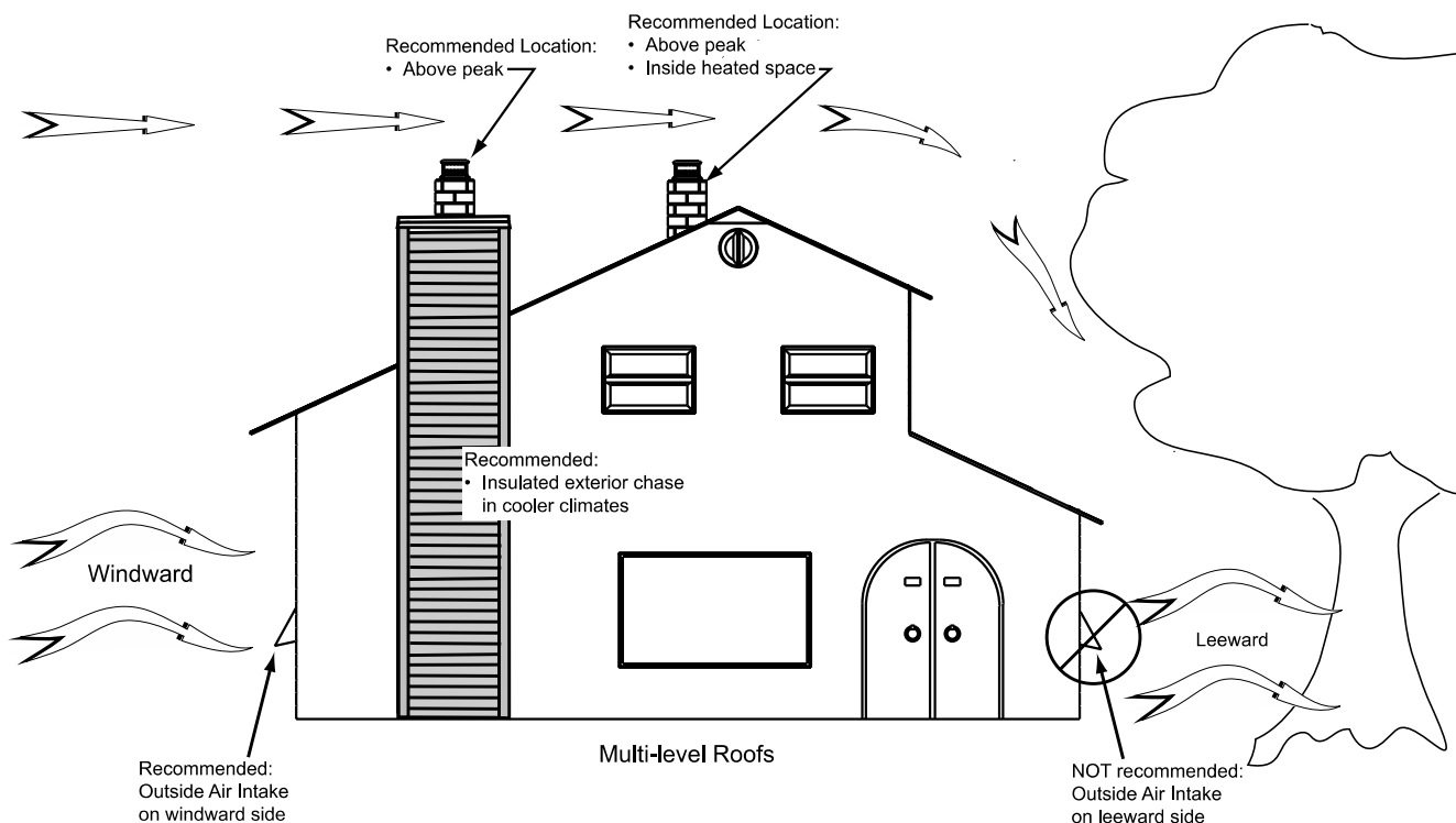
Figure 53: Air supply in conventional houses
