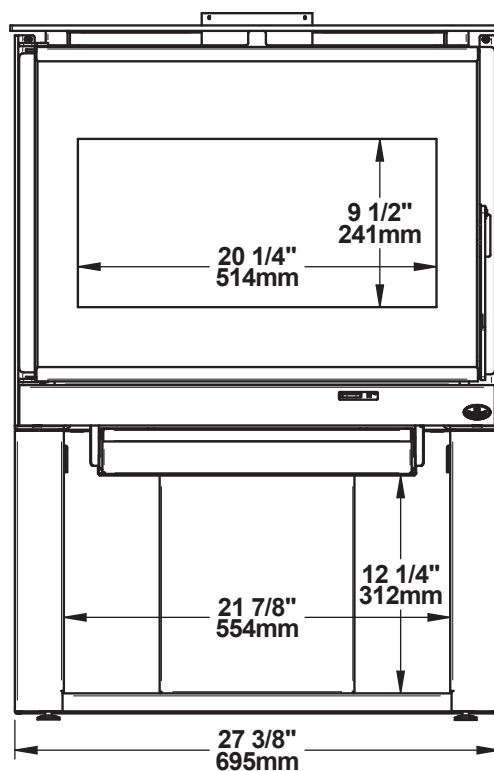
Figure 5: Front view
