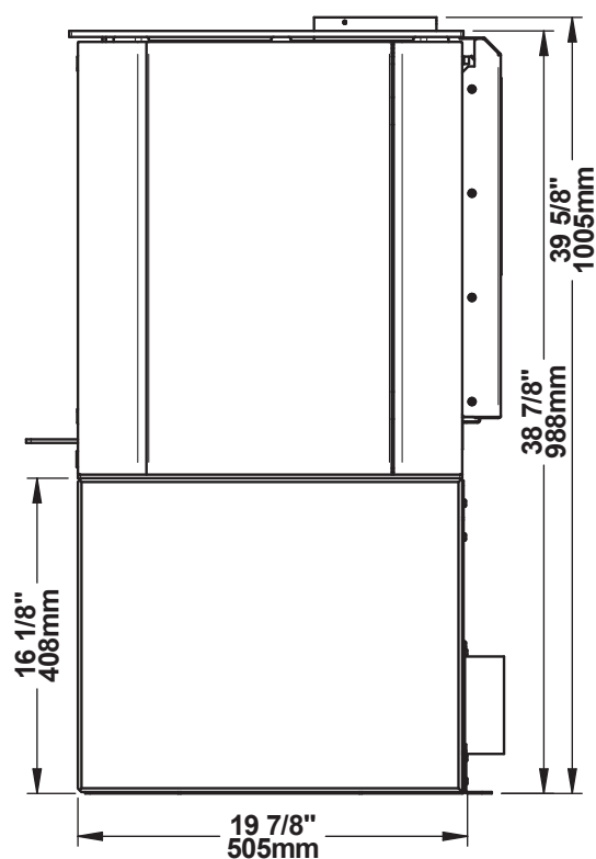
Figure 10: Side view
