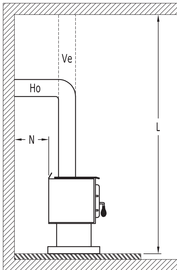
Figure 44: Clearances - Side
