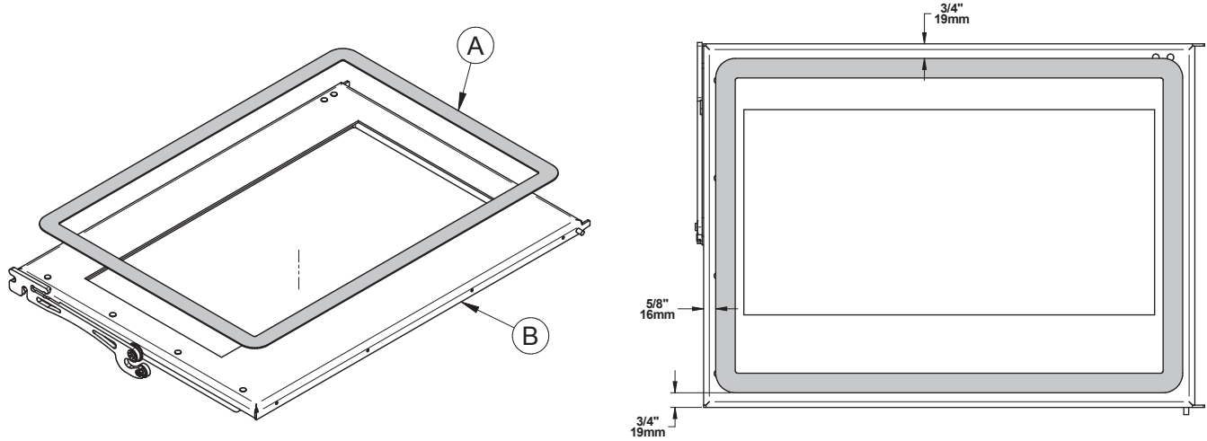
Figure 36: Replacing the glass gasket
