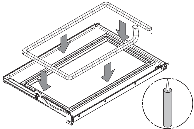
Figure 42: Door gasket
