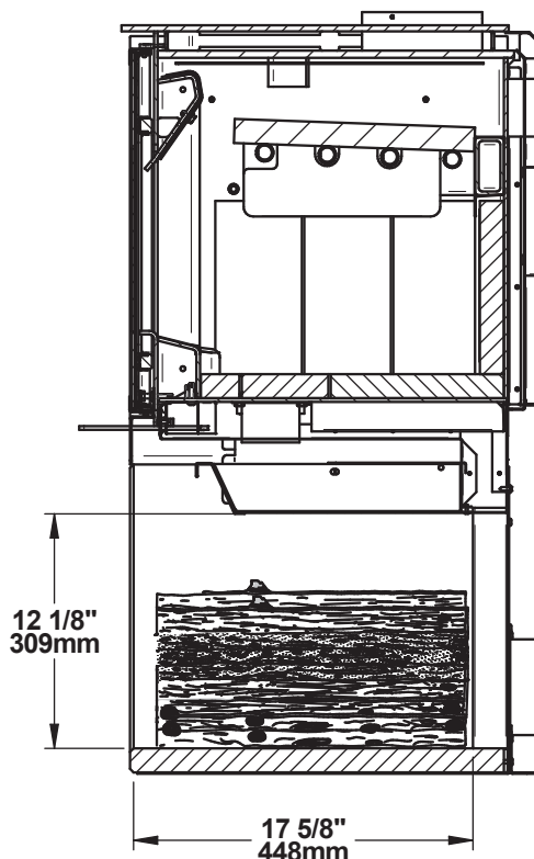
Figure 11: Side view
