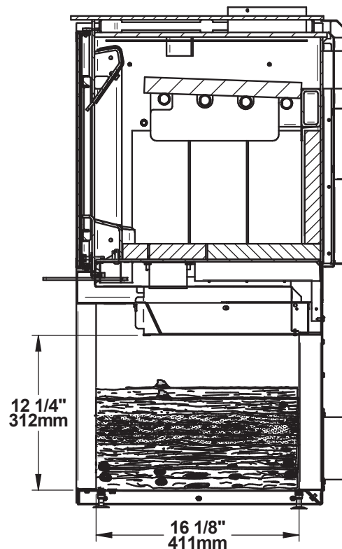
Figure 7: Side view
