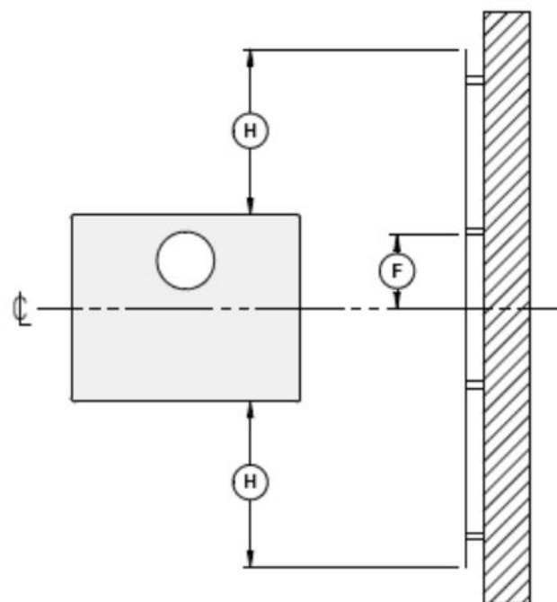
Figure 49: Heat shield clearances
