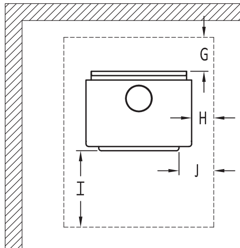
Figure 46: Floor Protection
