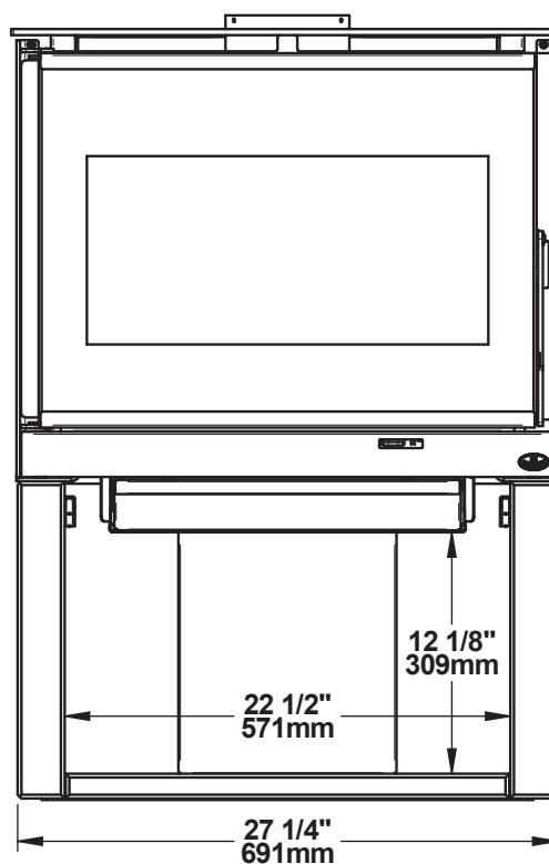
Figure 9: Front view
