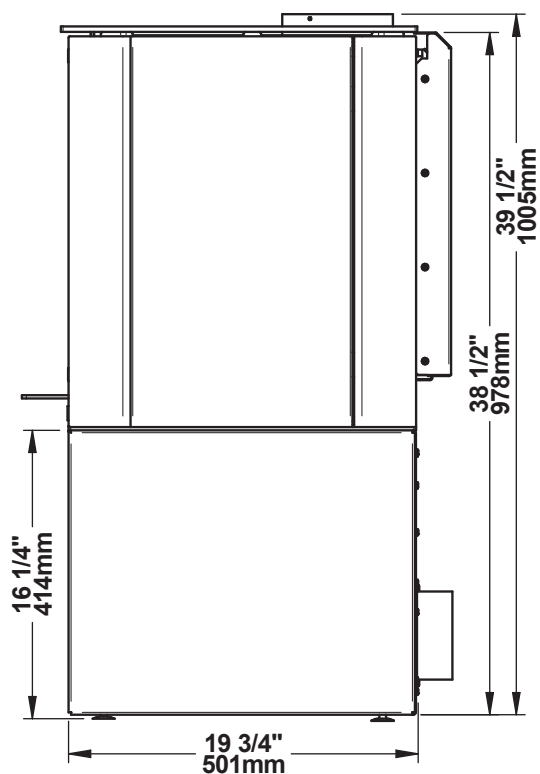
Figure 6: Side view
