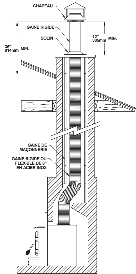
Figure 18: Installation de la gaine
