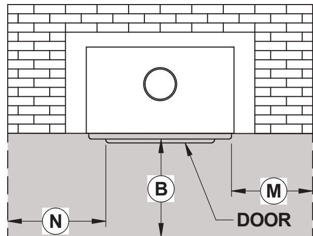
Figure 12: Protection de plancher
