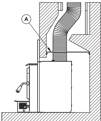
Figure 16: Plaque non combustible
